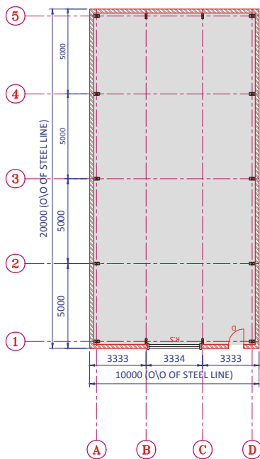
FLOOR PLAN 10x20x4.5M SMALL UNIT
