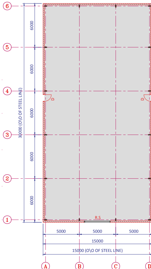
FLOOR PLAN 15x30x6M MEDIUM UNIT
