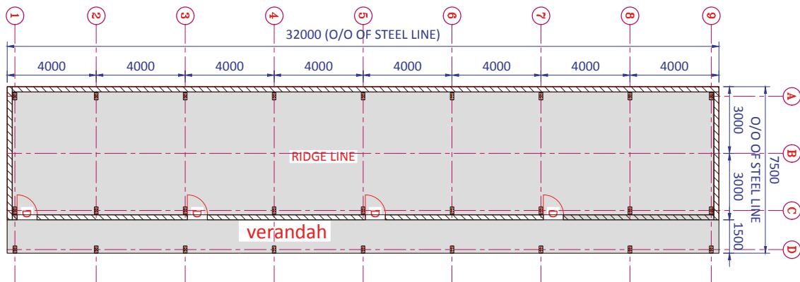
FLOOR PLAN 6x32x3M 4UNIT BLOCK
