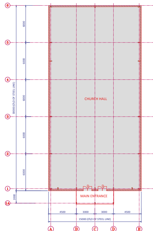
FLOOR PLAN 15x30x5M MEDIUM CHURCH
