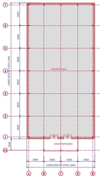
FLOOR PLAN 12x24x4M SMALL CHURCH
